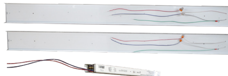
Back view. 8CK100 8 ft. LED Strip Light Conversion Kit with separate driver shown below.
