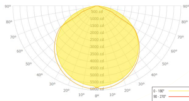
CANDELA POLAR PLOT OA212
