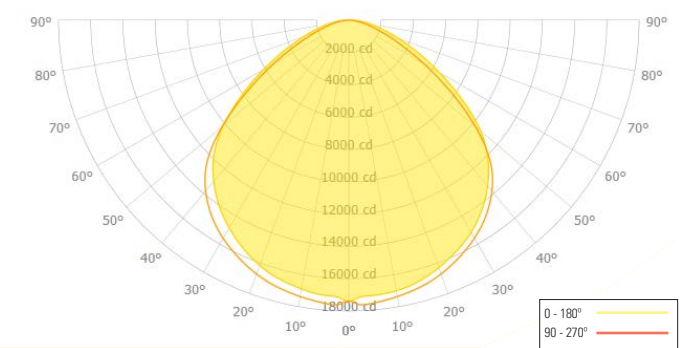
CANDELA POLAR PLOT OA436
